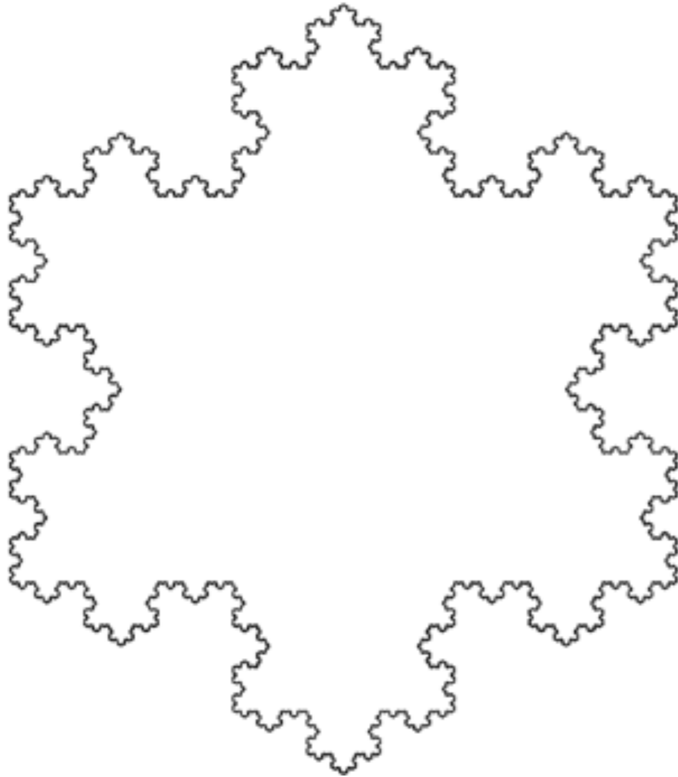
Koch snowflake
