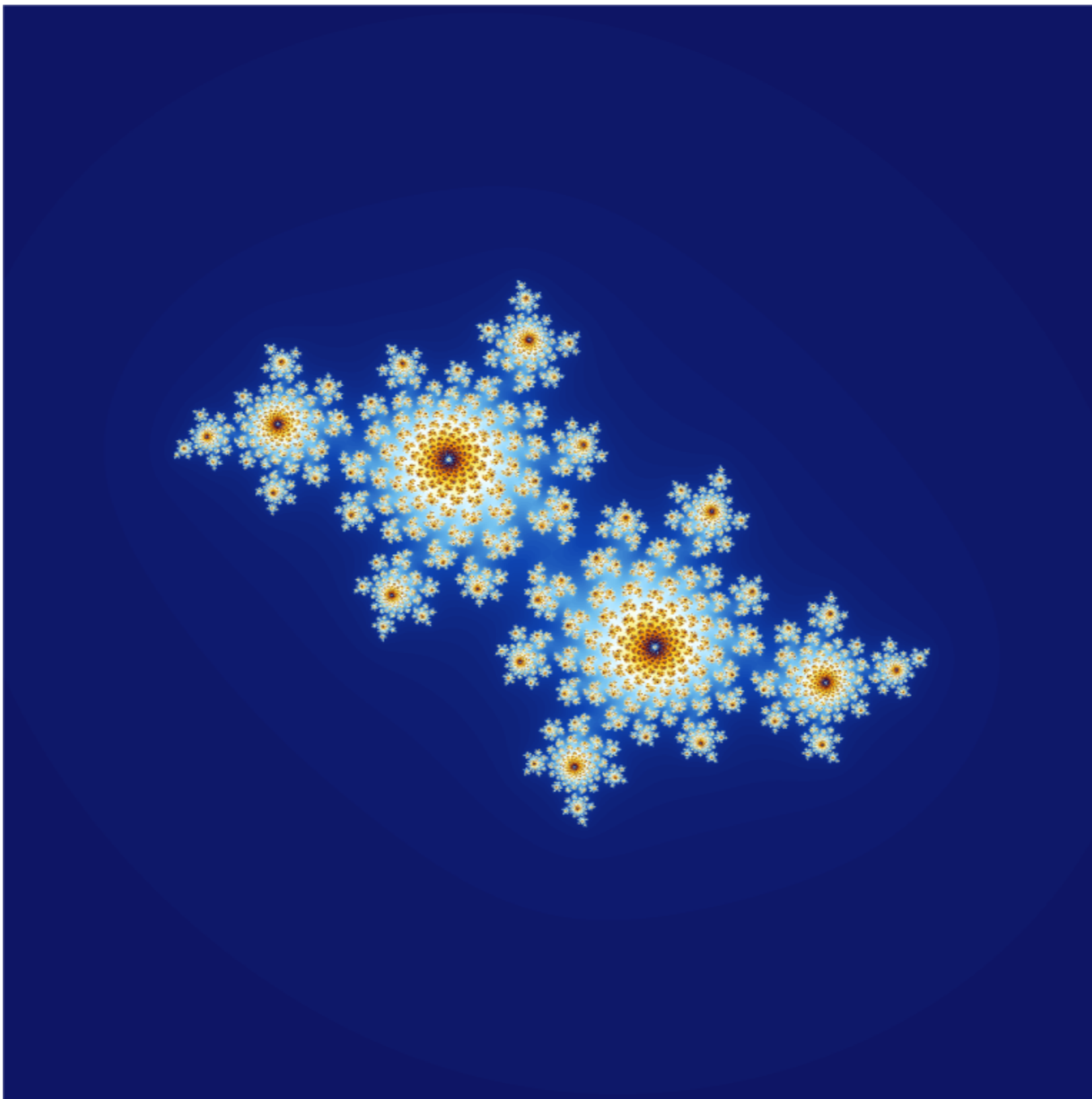
Julia set
