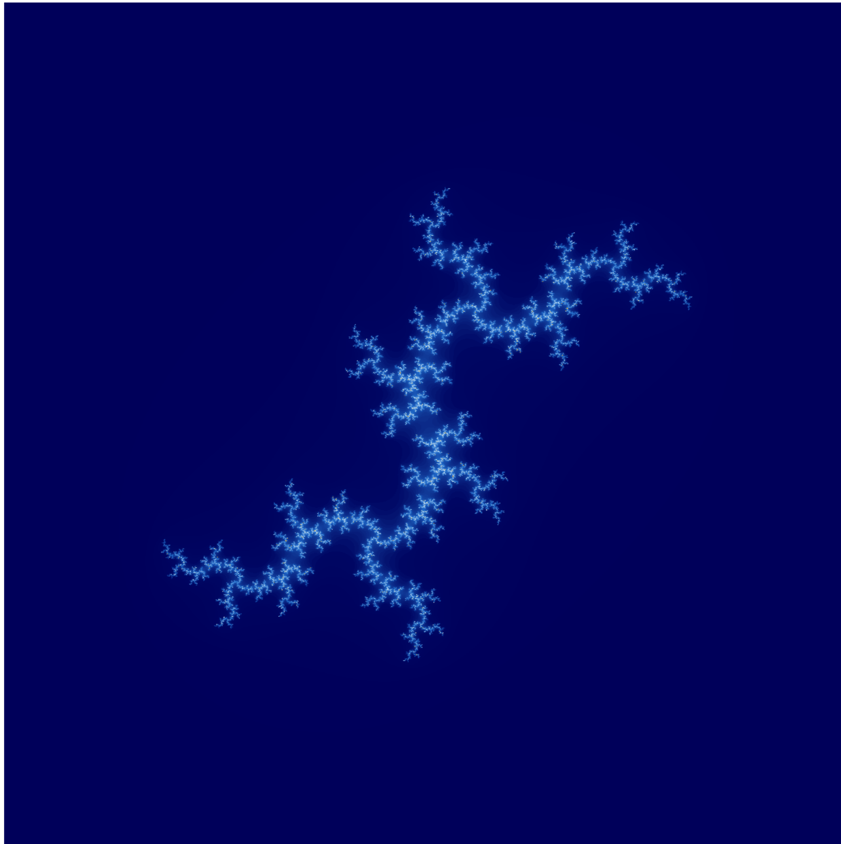
Julia set
