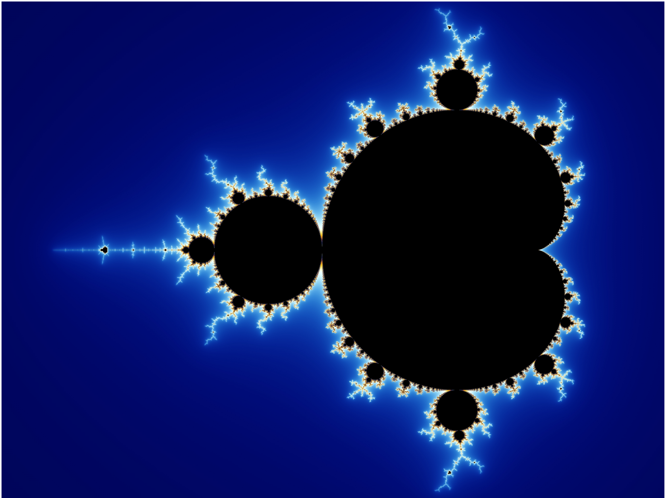
Mandelbrot set
